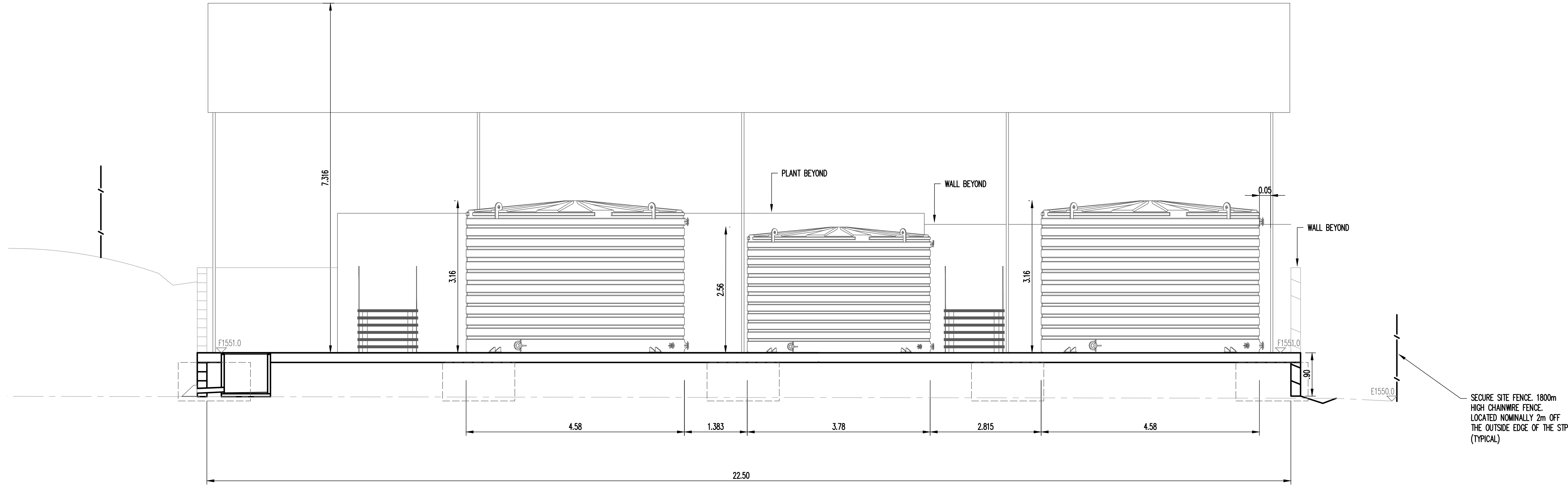
SECTION 1 SCALE 1:100
