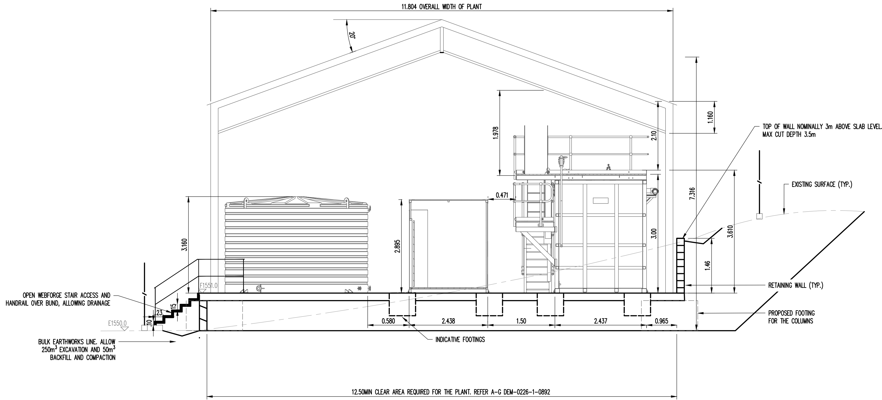
SECTION 2 SCALE 1:100
